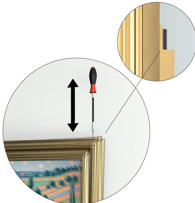
Adjust from top for parallel hanging
