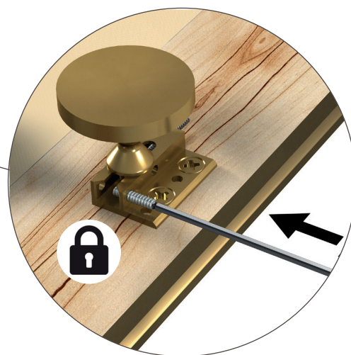
Tighten security screw to secure Depot Screw
